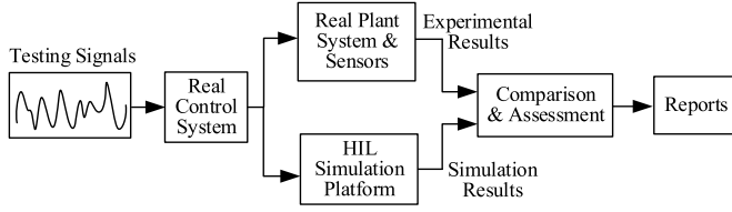
Fig. 15. Simulation credibility assessment experiments [17].
