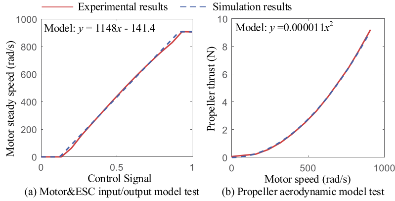
Fig. 14. Modeling accuracy verification of propulsion system with experiments and simulations.
