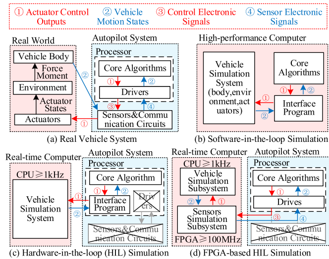
Fig. 1. Comparisons between common simulation methods.
