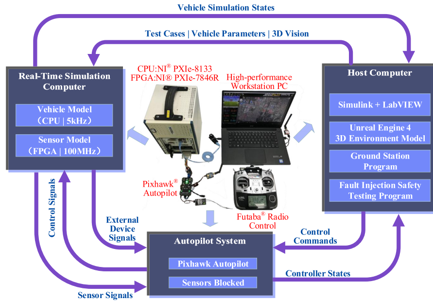
Fig. 9. Hardware composition of the real-time HIL test platform.
