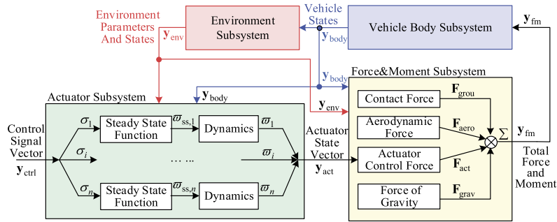
Fig. 5. The structure of the vehicle simulation subsystem.
