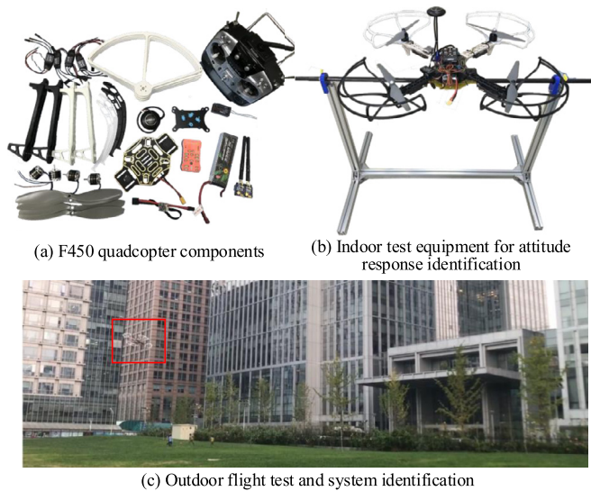
Fig. 13. Verification equipment for the proposed HIL test platform.
