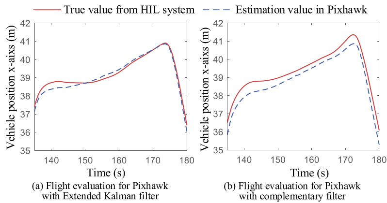
Fig. 17. Comparing estimation performance of different filter algorithms in turning flight stage.
