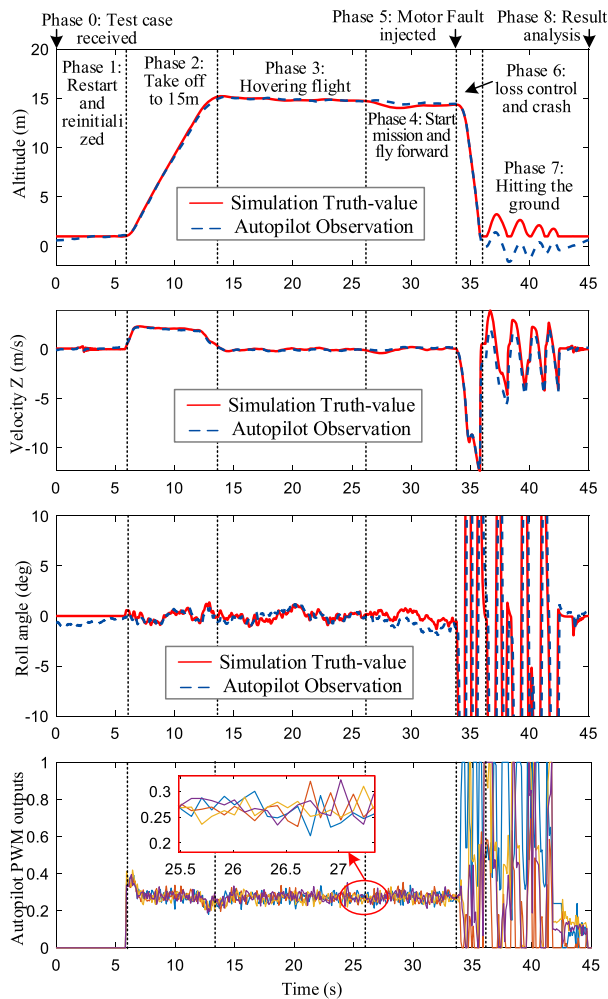
Fig. 19. Automatic test results of one motor failed case during the flight mission.
