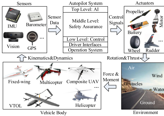
Fig. 3. System structure of unmanned aerial vehicles.
