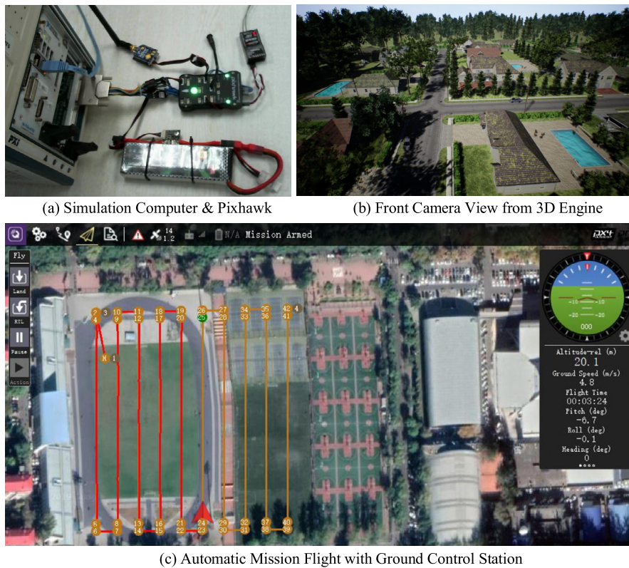
Fig. 18. Autonomous mission flight test with the proposed HIL test platform.
