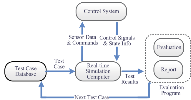
Fig. 12. Automatic safety testing and assessment framework.
