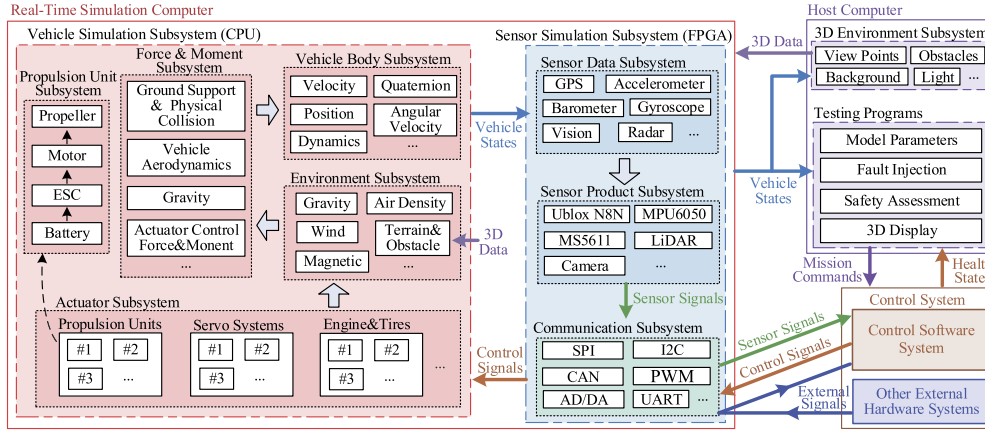
Fig. 4. System structure of the simulation test platform for UAV autopilot systems.
