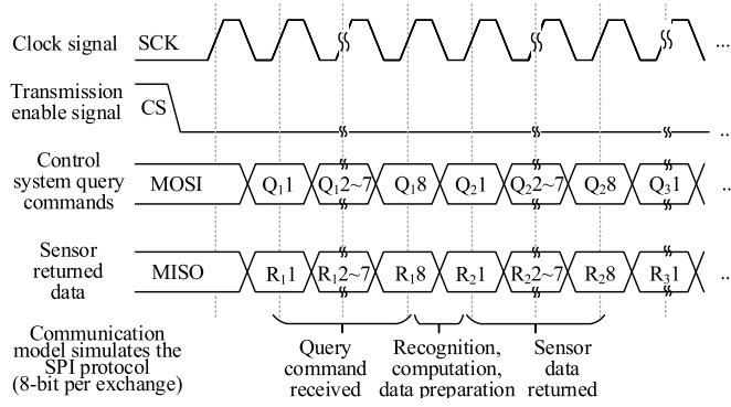
Fig. 7. Communication subsystem model for SPI buses.
